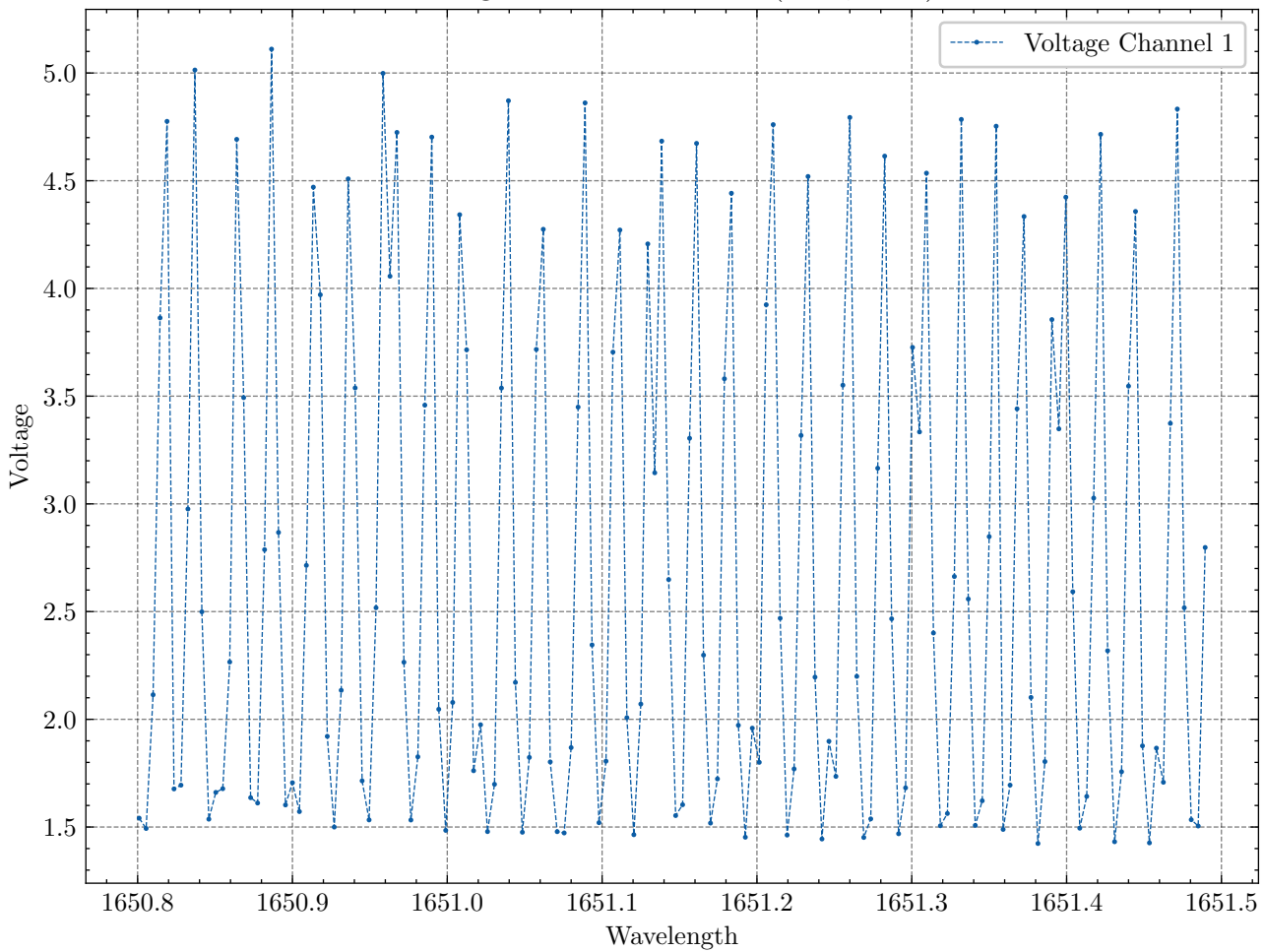
Voltage with Default LUT (5178, 5333)
